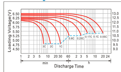
Discharge Characteristics Curve
