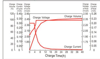
Charge Characteristics Curve
