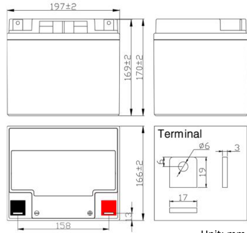
Unit: mm
